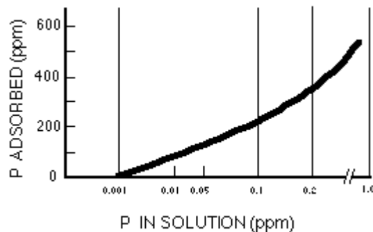
Figure 2. Relationship between P adsorbed by soil and P in solution.
